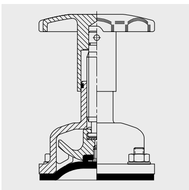
Stainless Steel 'Silicone sealed' Valve sizes: DN8 to DN80
