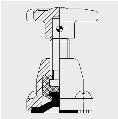
Rising Handwheel Valve sizes: DN8 to DN10
