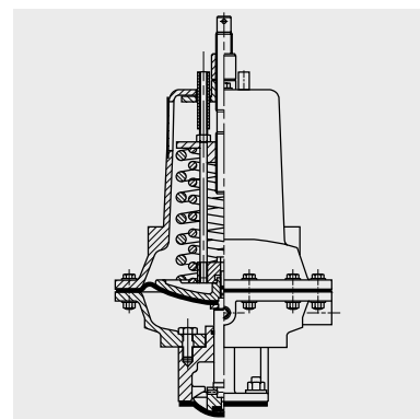
ES failsafe actuators (spring close/spring open/double acting) Valve sizes: DN8 to DN250
