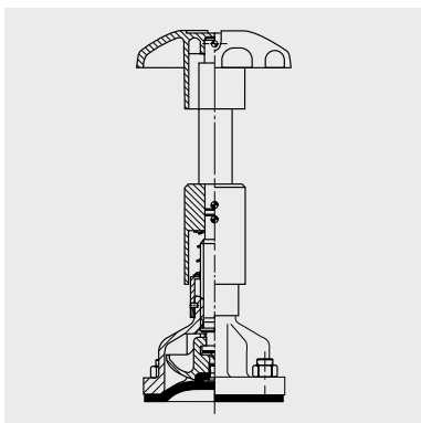
Extended Spindle (rising handwheel design changes to non-rising at DN200) Valve sizes: DN15 to DN350
