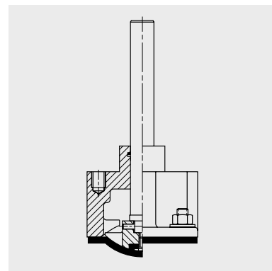
Sliding Spindle (for use with proprietary actuator) Valve sizes: DN15 to DN350
