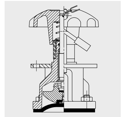
Viton Sealed Padlocking Valve sizes: DN15 to DN150
