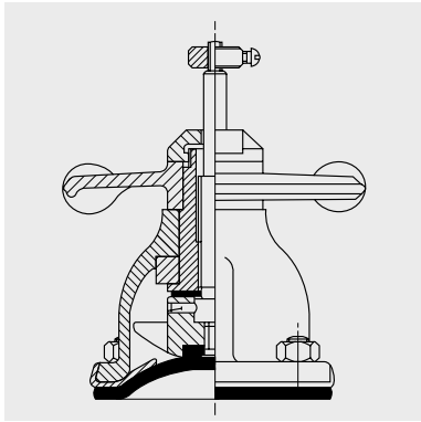
Cast Steel Rising Spindle Indicator (with limit stop) Valve sizes: DN15 to DN300
