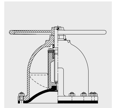
Non-rising Handwheel Valve sizes: DN200 to DN350
