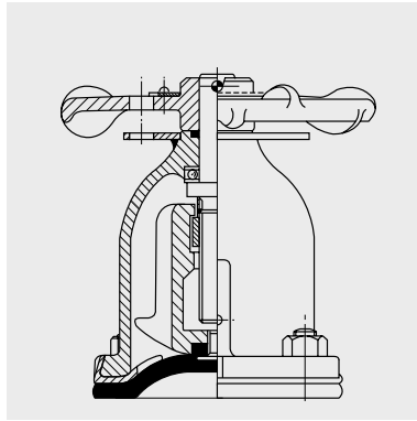
Non-rising Gunmetal LG4 Padlocking Valve sizes: DN15 to DN200
