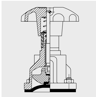
Viton Sealed Bonnet Valve sizes: DN15 to DN150
