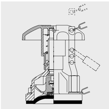
Rising Handwheel Indicator (simple padlocking) Valve sizes: DN15 to DN150
