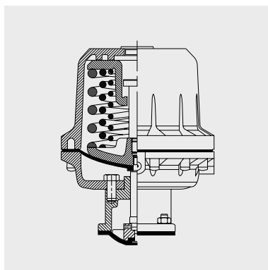
ECX actuator (spring close/spring open/double acting) Valve sizes: DN65 to DN150
