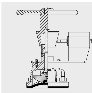
Rising Handwheel with microswitch Valve sizes: DN25 to DN150
