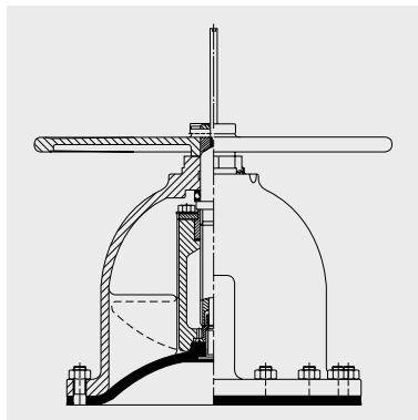
Non-rising Handwheel with Indicator Valve sizes: DN200 to DN300
