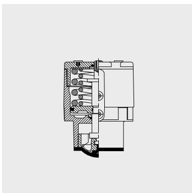
EC actuator (spring close/spring open/double acting) Valve sizes: DN8 to DN50
