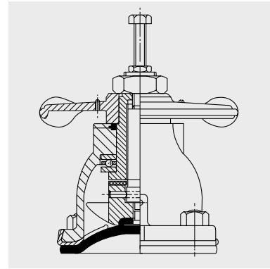
Non-rising Gunmetal LG4 Limit opening Valve sizes: DN15 to DN150
