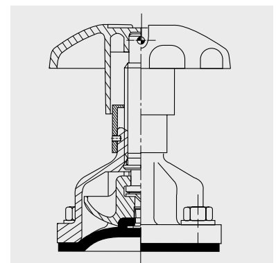
IXEF Polyamide Bonnet Valve sizes: DN15 to DN50
