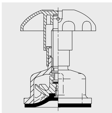
Stainless Steel 'Non-sealed' Valve sizes: DN15 to DN80
